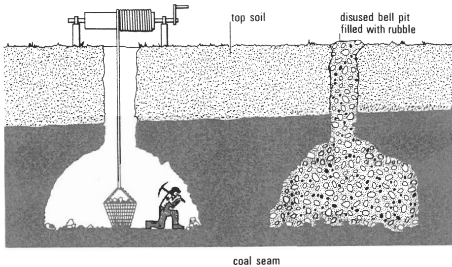
Figure 1. Bell Pit (from Technological Essay: Coal . Open University Press 1983)
